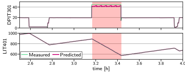
(b) Having identified the potential attack points, a closer investigation of the predicted and measured behavior gives further insights into the attack. Here, DPIT301 behaves differently than predicted.
