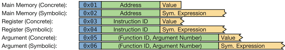
Fig. 2. Six kinds of fragments suffice to denote all possible variants. Symbolic values are written as serialized symbolic expressions consisting of all relevant constraints. All other fields only ever contain concrete values, which are simply used verbatim. Fields of dynamic size are denoted by a ragged right edge.
