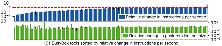
Fig. 5. BusyBox, 60 min time limit. Relative change of instructions per second (top) and peak resident set (bottom) versus the KLEE baseline. Note the logarithmic scale and the black 99% confidence intervals.
