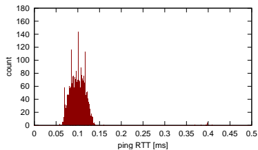
(a) RTTs for two Linux PCs
