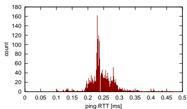
(c) Synchronized execution of one virtualized host and a simulation
